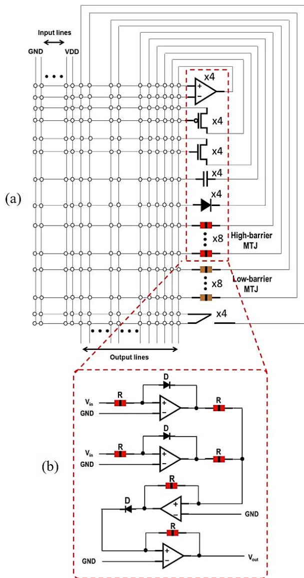
Fig. 4: (a) M-FPAA CAB structure and (b) configuration of an analog multiplier circuit using CAB elements.
