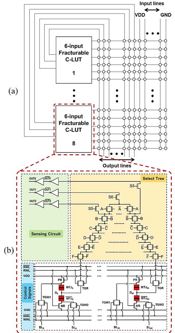
Fig. 3: (a) M-FPAA CDB structure and (b) C-LUT circuit components utilized for CDB logic select/retrieval [2].
