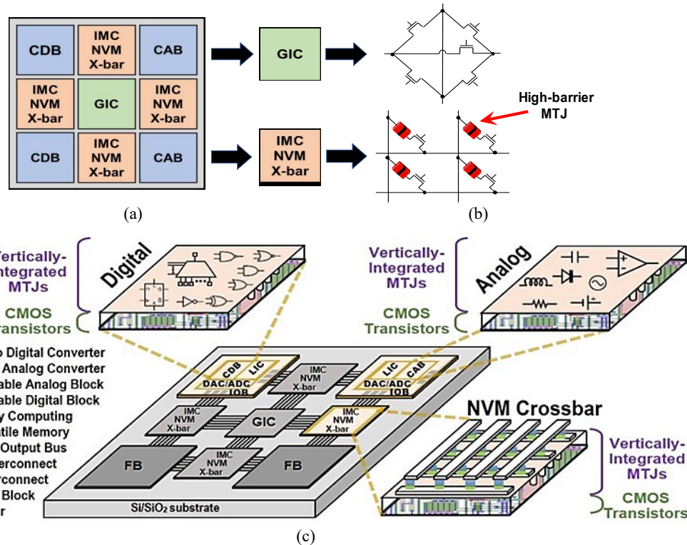
Fig. 1: (a) Single-Slice organization for proposed M-FPAA architecture, (b) M-FPAA routing and switch interconnect design, and (c) Hybrid Spin/Charge device realization as configurable blocks within the M-FPAA fabric.
